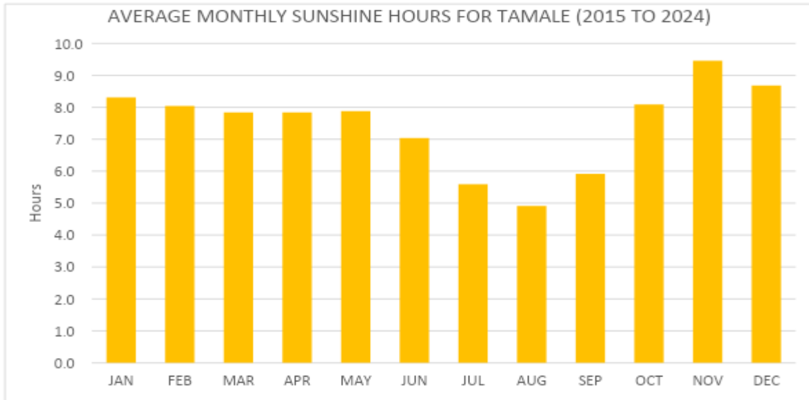
Figure 5-6: Average Total Sunshine Hours
