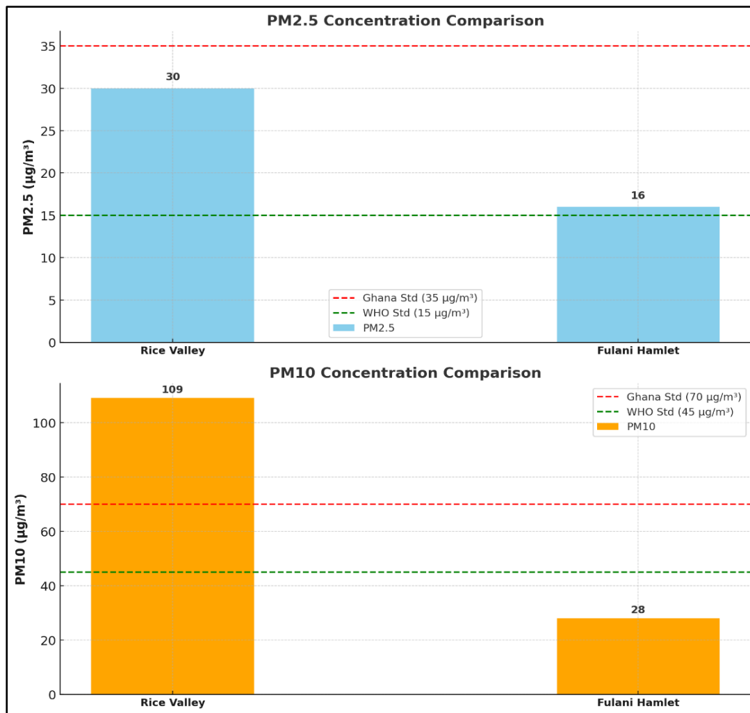
Figure 5-14: Graph showing compliance and or exceedance of particulates to GSA/WHO Standards (SAL Consult, 2025)
