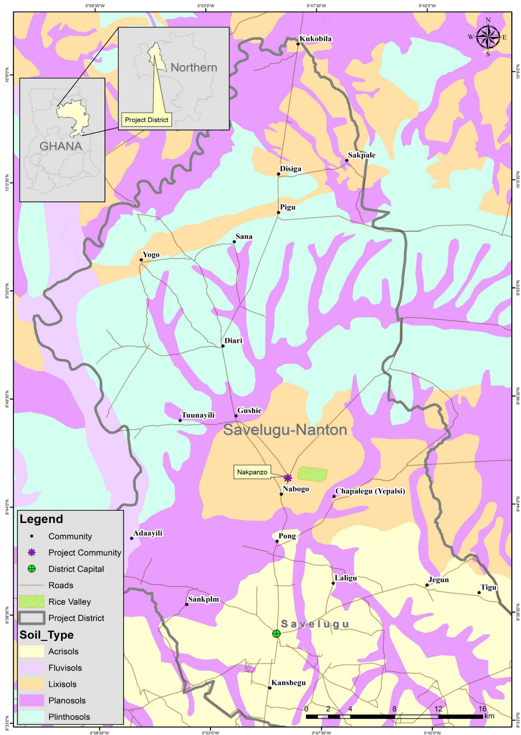
Figure 5-12: Geology Map of the Savelugu Municipal (Source: SAL Consult, 2025)
