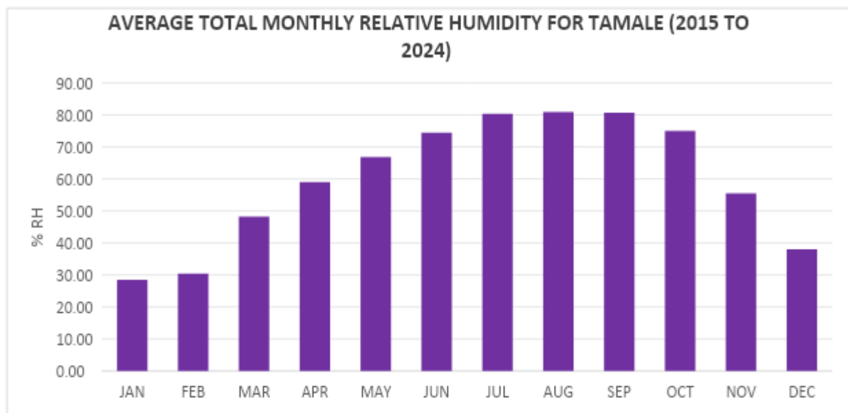
Figure 5-5: Average Monthly Relative Humidity (Ghana Meteorological Agency, 2025)
