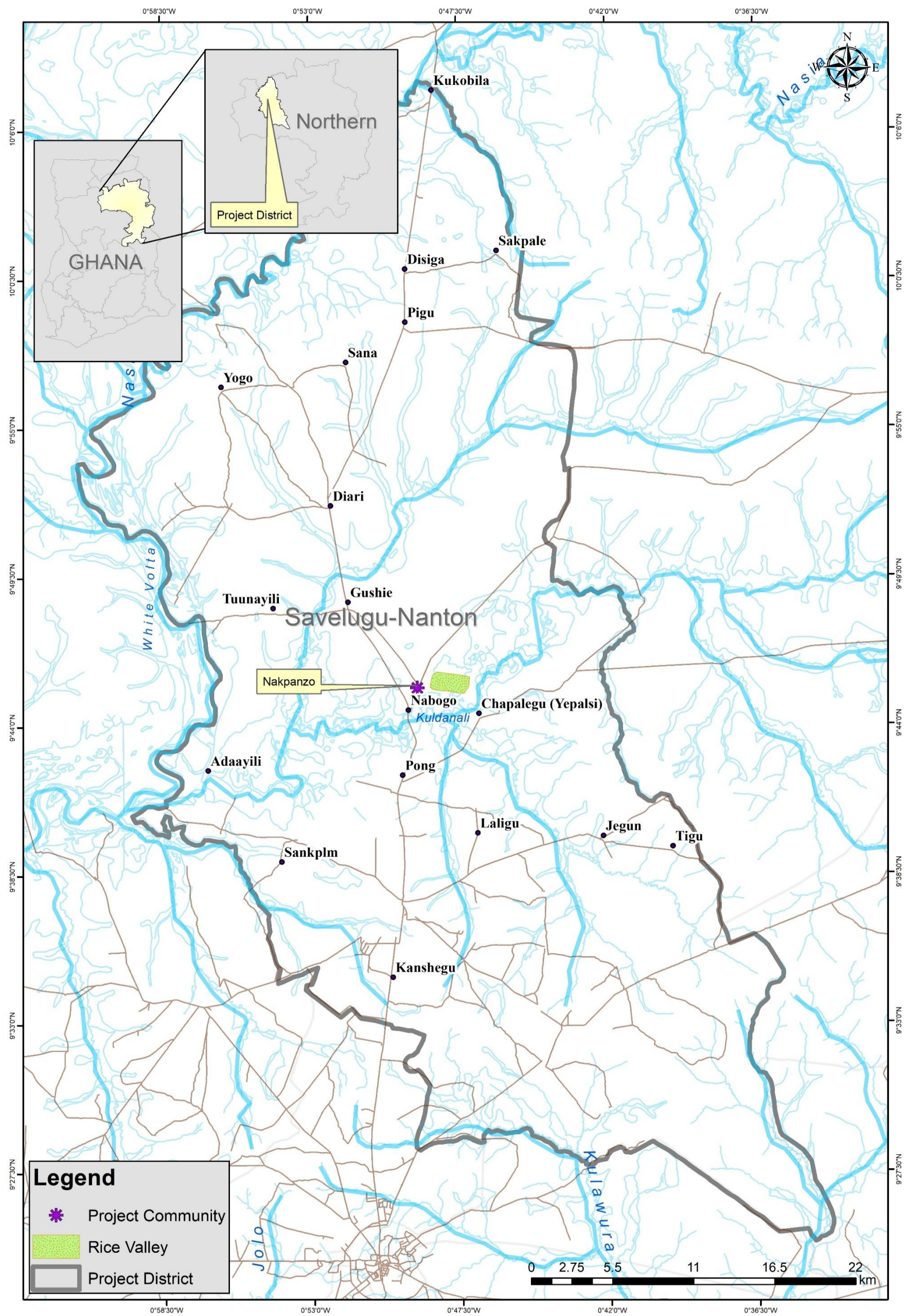
Figure 5-10: Drainage Map of the Savelugu Municipal (Source: SAL Consult, 2025)
