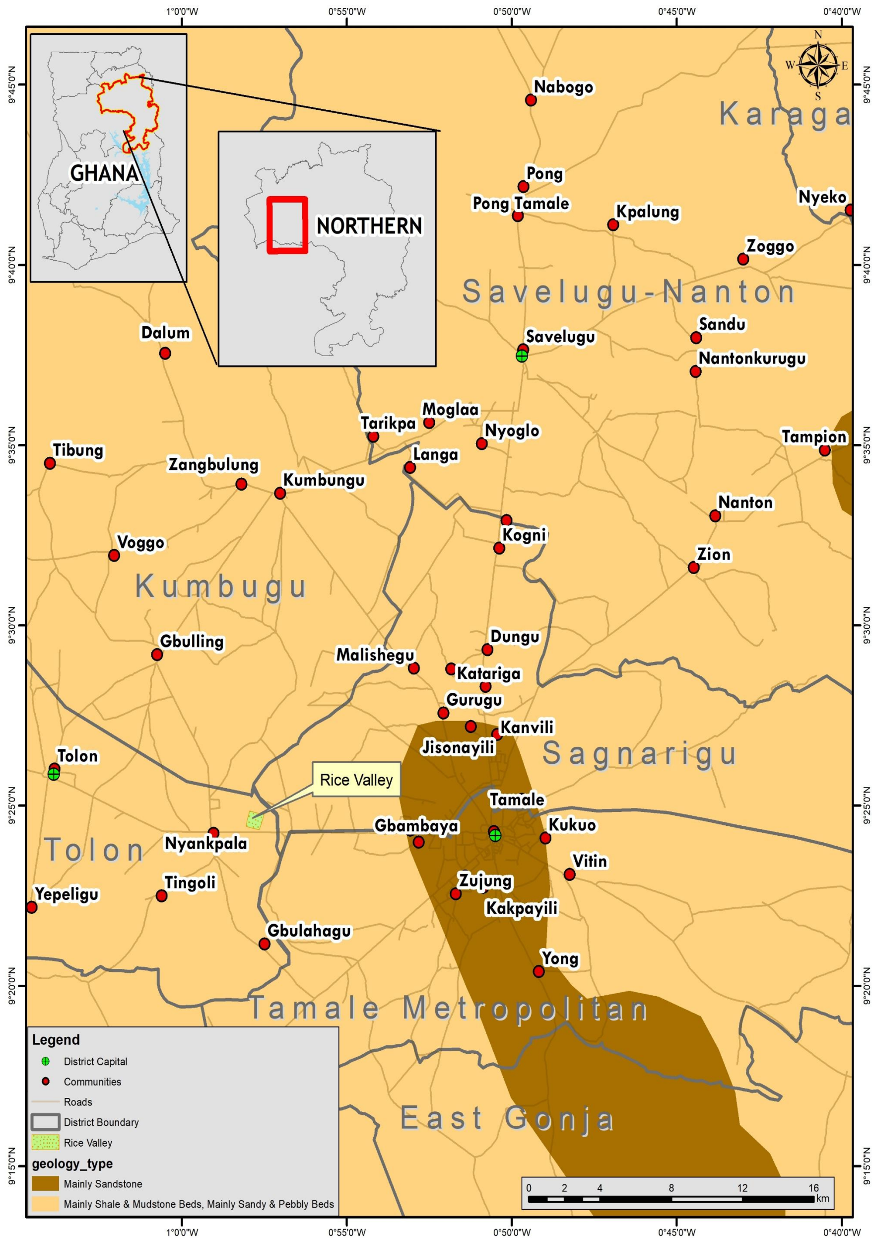
Figure 5-10: Geology Map of the Tamale Metropolitan (Source: SAL Consult, 2025)
