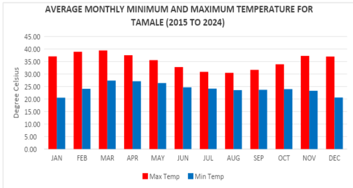
Figure 5-4: Average monthly Minimum and Maximum temperature
