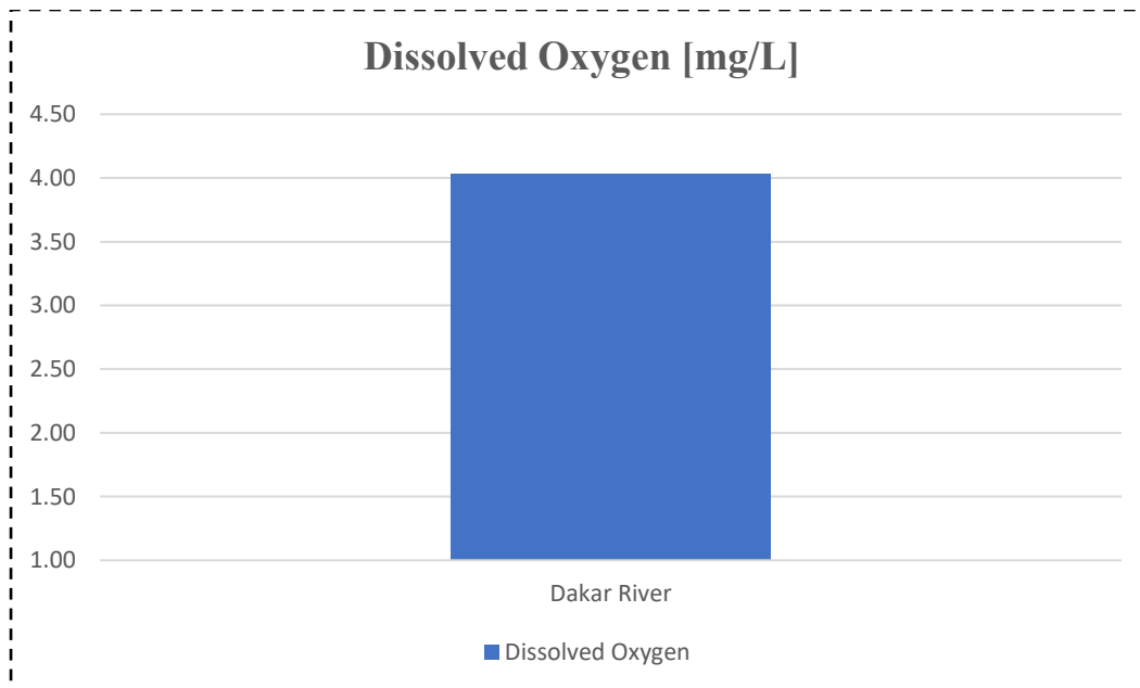
Figure 5-19: Graph showing In-situ measurement of dissolved oxygen (SAL Consult, 2025)
