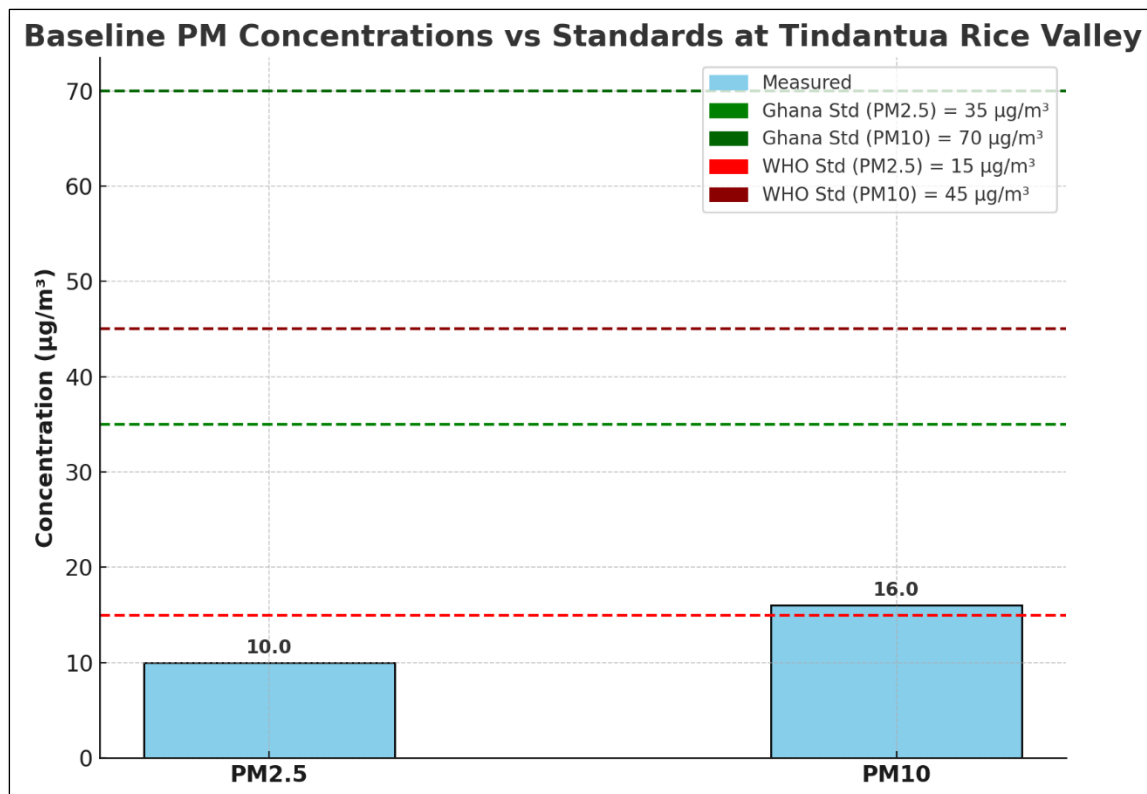
Figure 5-13: Graph showing compliance and or exceedance of particulates to GSA/WHO Standards (SAL Consult, 2025)
