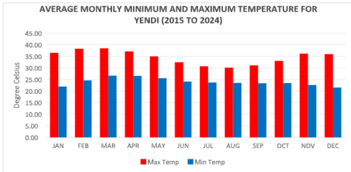
Figure 5-4: Average monthly Minimum and Maximum temperature (Ghana Meteorological Agency, 2025)
