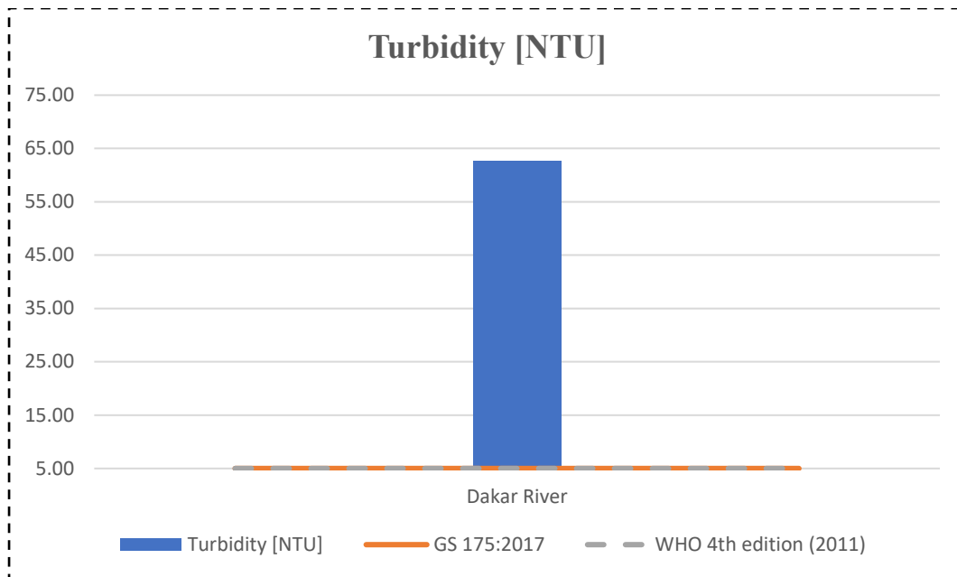
Figure 5-20: Graph showing In-situ measurement of Turbidity (SAL Consult, 2025)
