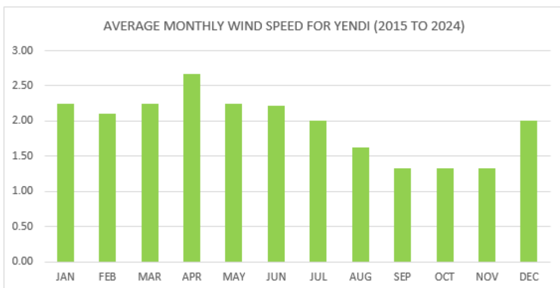
Figure 5-7: Average Monthly Wind Speed
