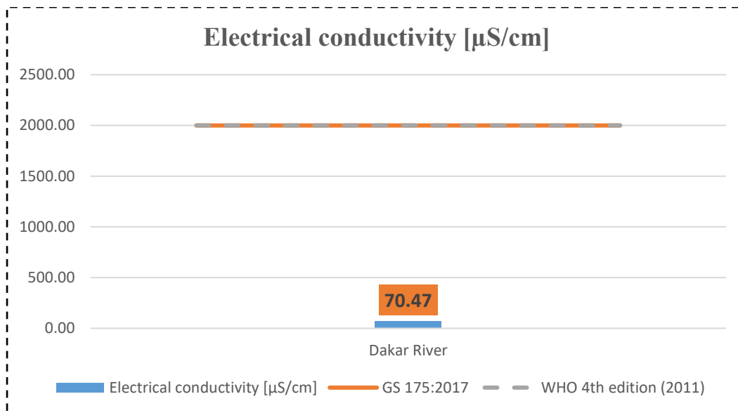
Figure 5-17: Graph showing In-situ measurement of electrical conductivity (SAL Consult, 2025)
