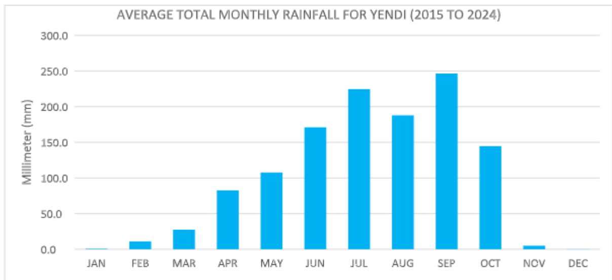
Figure 5-3: Average Monthly rainfall
