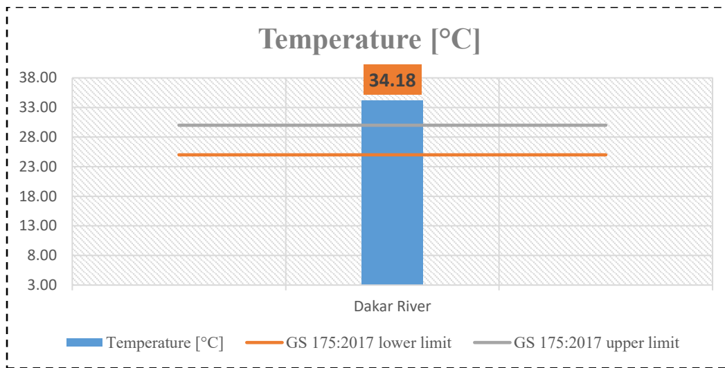
Figure 5-15: Graph showing In-situ measurement of temperature (SAL Consult, 2025)
