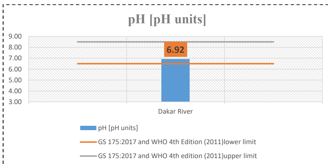
Figure 5-16: Graph showing In-situ measurement of pH
