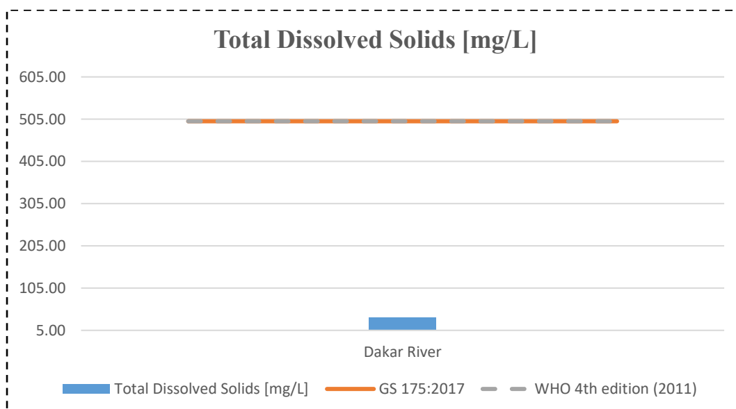
Figure 5-18: Graph showing In-situ measurement of total dissolved solids (SAL Consult, 2025)
